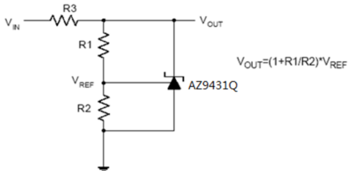
Shunt Regulator
